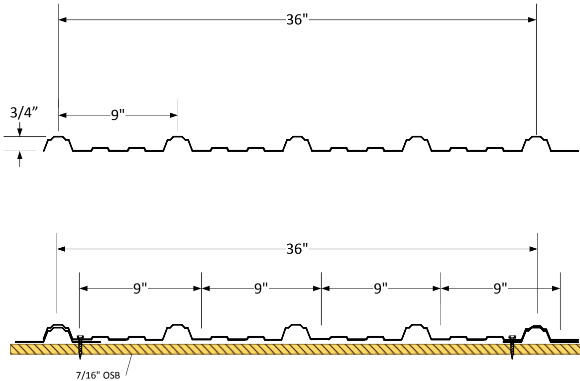
FASTENER PATTERN @ 6" O.C.
